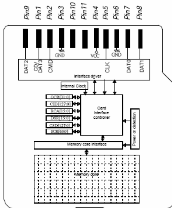
Fig. 1-1 miniSD memory card system diagram
